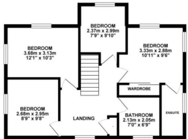
1ST FLOOR 52.23 sq. m. ( 562.17 sq. ft. )
